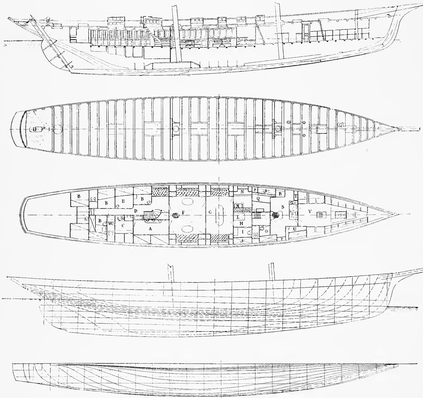
THE CELEBRATED FRENCH SCHOONER YACHT VELOX.—Built by M. A. Normand, Havre.
